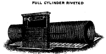
FULL CYLINDER RIVETED WITH LAP JOINT CONSTRUCTION REINFORCED ENDS, BEST MADE
